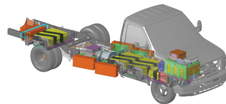
MOTIV-POWERED FORD E-450 CHASSIS
